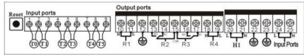
controller SR618C6, schema 11
